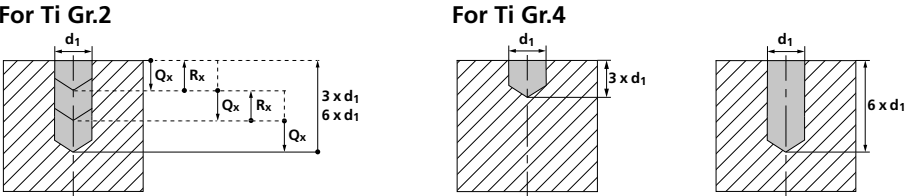
Chip breaking cycle (e.g.: G73)
